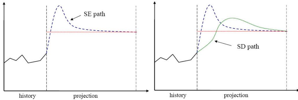
Figure 2: Short-run equilibrium (SE) and short-run dynamic (SD) path
